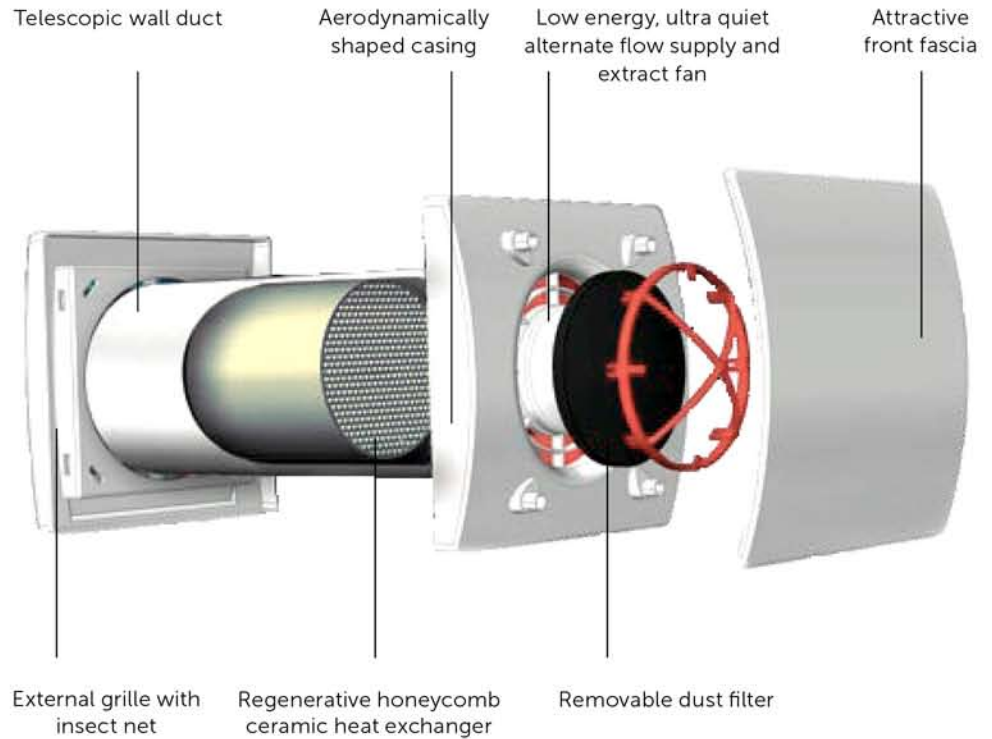
Unit on extraction and heat retention mode
